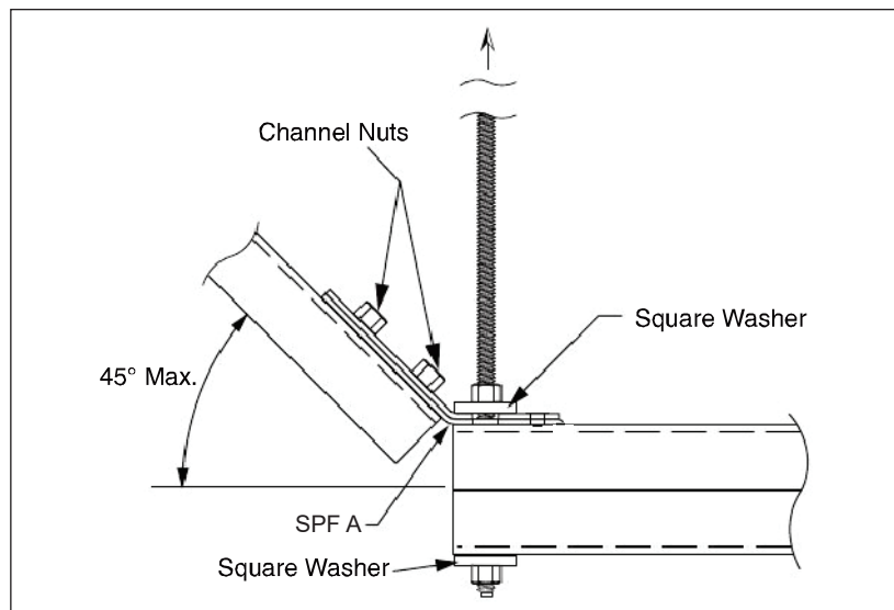
Transverse Brace
