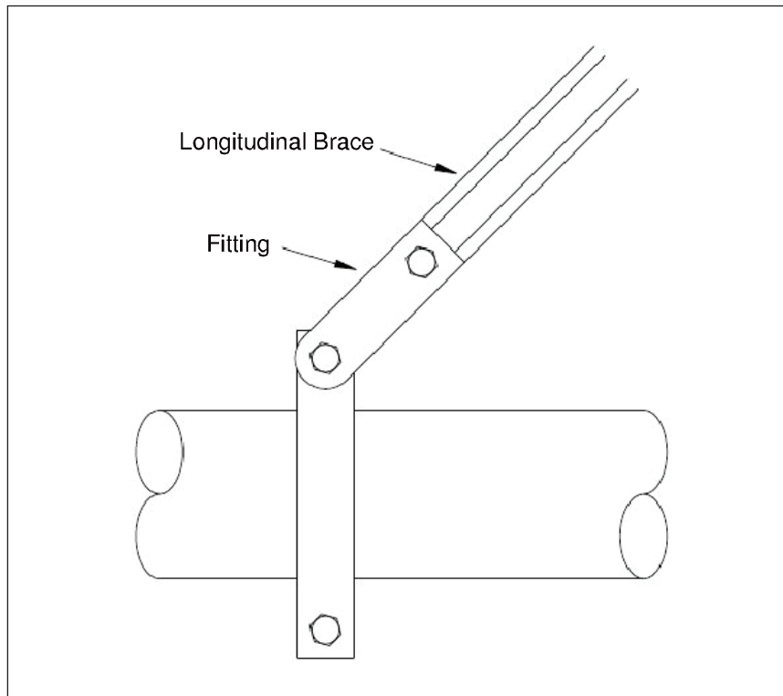
Transverse Brace
