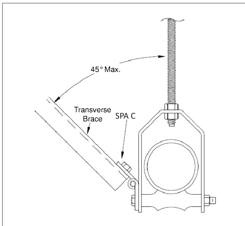
Transverse Brace
