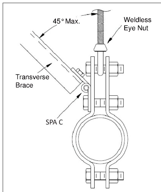
Transverse Brace
